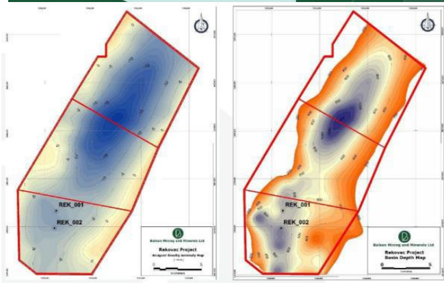
Rekovac project terrain corrected Complete Bouguer gravity image contoured at 1m Gal (left) and computed basin depth image contoured at 50m (right).
