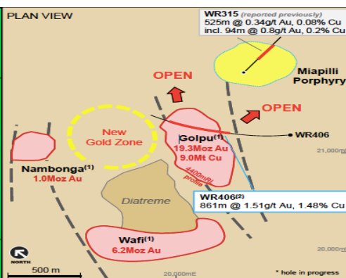
Wafi Resource Plan view. Current resource is stated at 460 MT @0.77 g/t Au & 0.81% Cu for 11.4 Moz Au & 3.73 Mt Cu (From Newcrest Mining Website)
